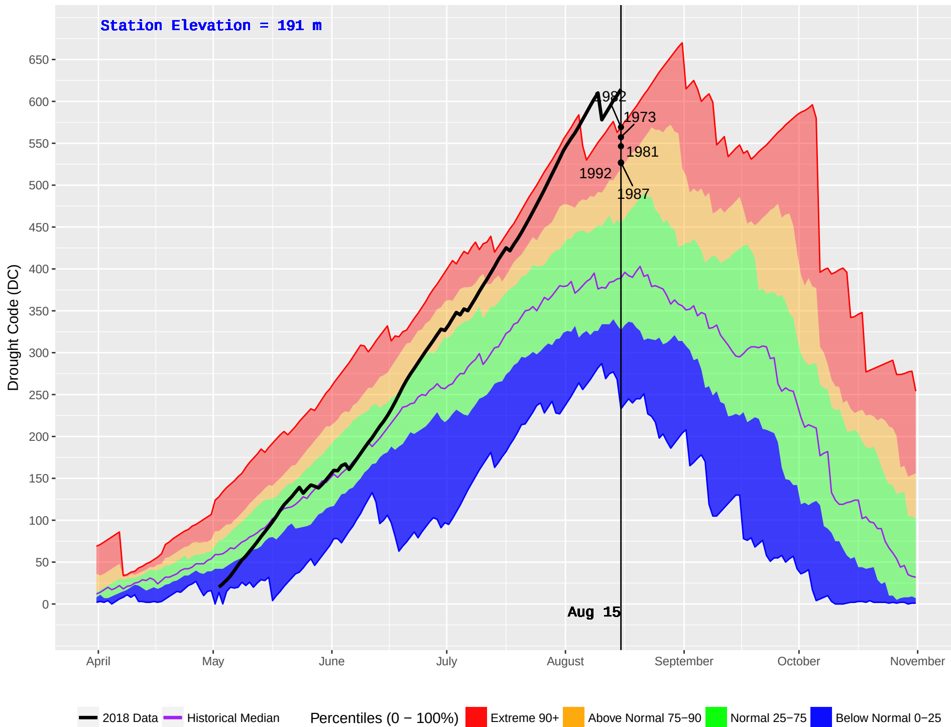
NASS CAMP (427) : Historical (1970–2016) and Current (2018) Daily Drought Code (DC)
